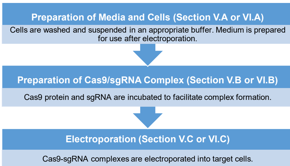
Figure 1. Protocol overview for Guide-it Recombinant Cas9 (3 µg/µl).
